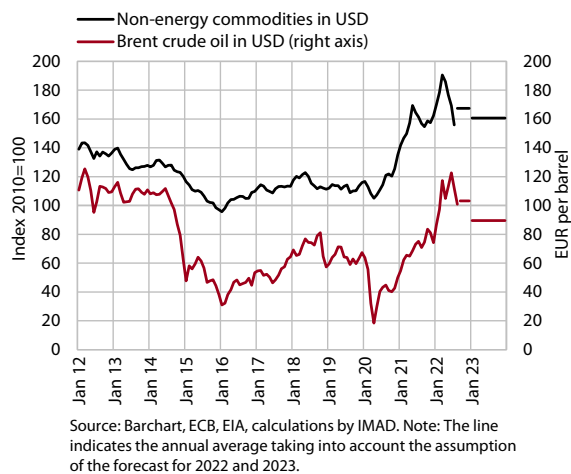
Figure 5: Prices of oil and non-energy commodities have fallen in recent months but still remain high
