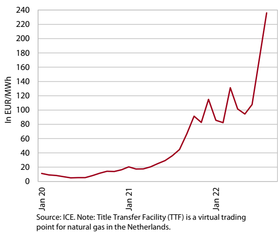
Figure 6: TTF gas prices rose to record levels
