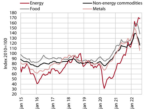
Figure 2: After falling in the summer months, prices of non-energy commodities remain high
